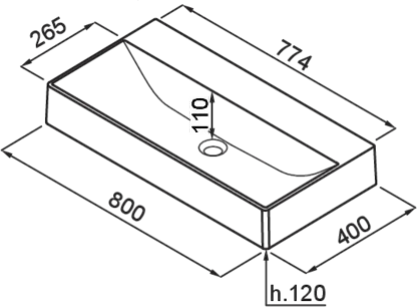
Technical Drawing
